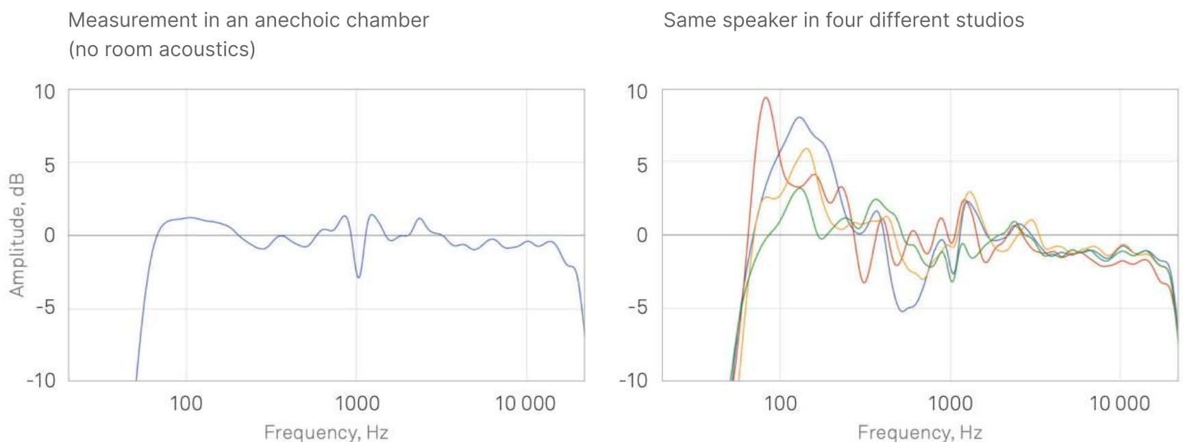
Figure 4: Speaker FR changes significantly when placed in a room
