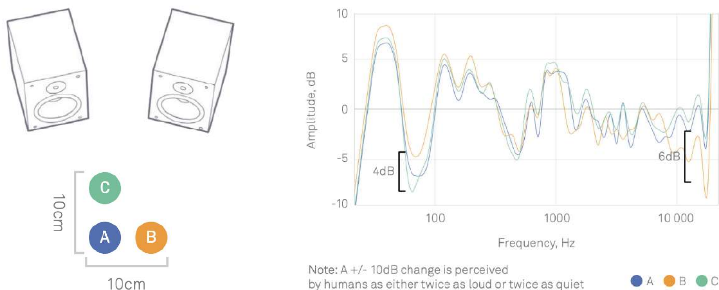
Figure 6: Speaker FR is uneven in a room. The same speakers measured in three different studio positions (10 cm apart).
