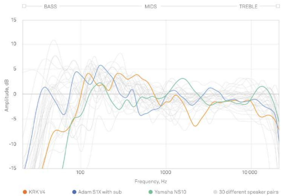
Figure 2: Frequency response variation of studio speakers 33 measured studio speaker pairs in various listening environments
