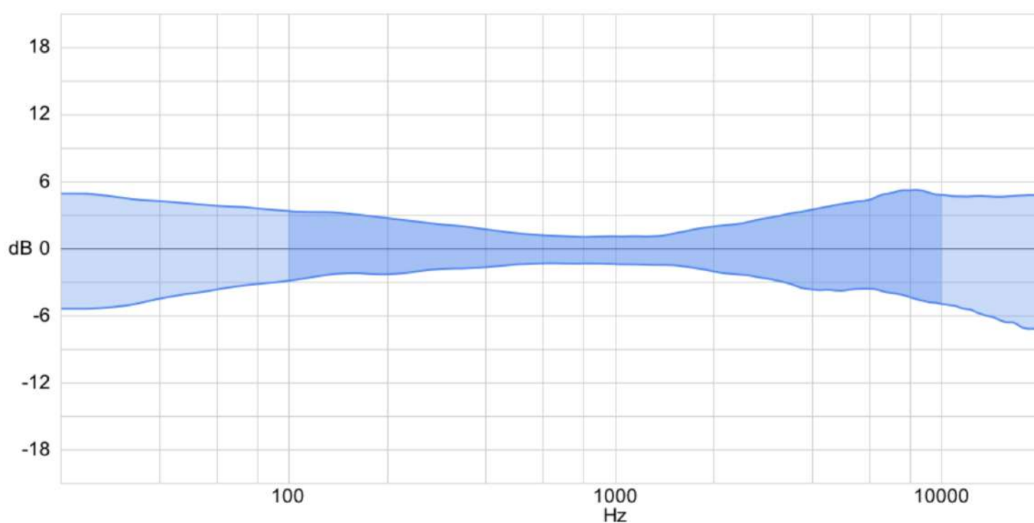
Figure 8: Figure 8. 90% confidence interval for individual deviation of Sonarworks calibrated headphone frequency response from the neutral reference by a panel of expert listeners.
